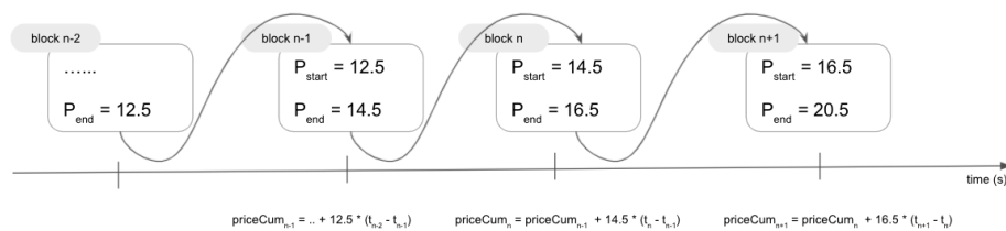
Fig. 1: NFT cumulative price on Blockchain. The initial price of an NFT in the next block is equal to the final price of the same NFT in the previous block
